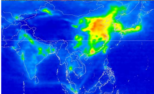
Atmospheric Spectrometry
